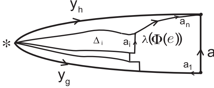
FIGURE 4. Van Kampen diagram \Delta_e for recursive edge e
