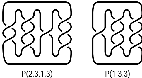
Figure 1: Pretzel knots
