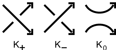
Figure 5: HOMFLY polynomial
