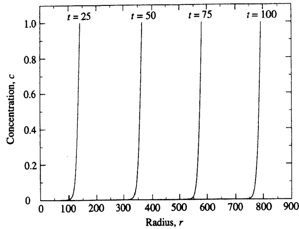
FIG. 3. The nutrient concentration plotted against radius for four values of t .
