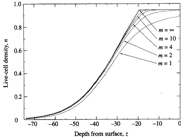
FIG. 7. Plots of the live-cell density against the tumour depth for five values of the exponent m = m_1 = m_2 .
