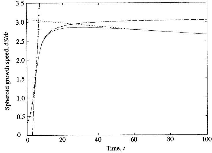
FIG. 11. Plots of growth speed against time for \varepsilon = 0.01 : (—) the numerical solution to the full system and asymptotic approximations for (— × —) the early time scale, (— · —) the mid time scale, and (· · ·) the long time scale.
