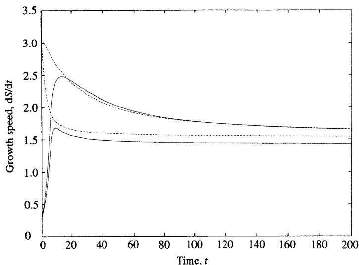
FIG. 14. Plots of the growth speed against time showing the numerical solution of (—) the full model and (---) the long-time solutions for \varepsilon = 0.1 (upper curves) and \varepsilon = 1 (lower curves).
