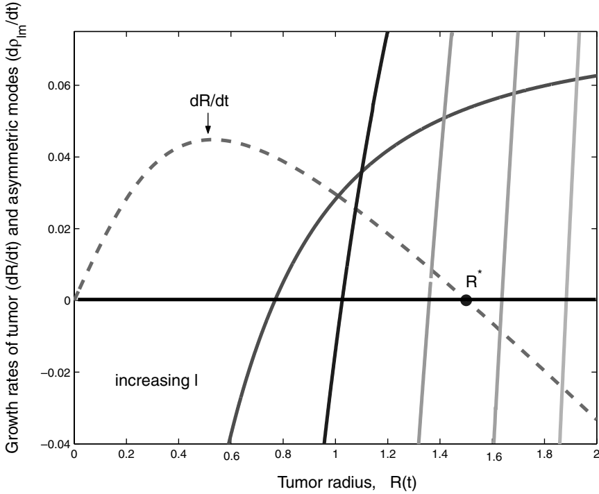
Fig. 2. The growth rate of asymmetric modes ( \frac{d\rho_{lm}}{dt} ) is plotted against the tumor radius for various choices of l ( l = 1, 2, 5, 10, 15, 20 ). The growth rate of the tumor is also plotted against R to show when asymmetric instability arises.
