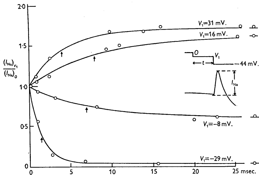
Fig. 3. Time course of inactivation at four different membrane potentials. Abscissa: duration of conditioning step. Ordinate: circles, sodium current (measured as inset) relative to normal sodium current; smooth curve, y = y_{\infty} - (y_{\infty} - 1) \exp(-t/\tau_h) , where y_{\infty} is the ordinate at t = \infty and \tau_h is the time constant (shown by arrows). Experimental details as in Figs. 1 and 2.
