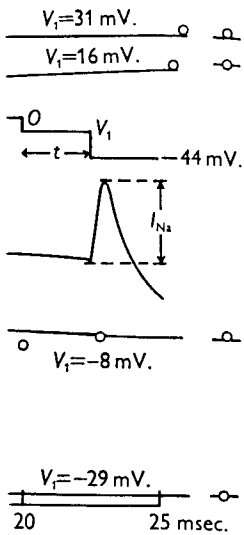
ntials. Abscissa: duration of l as inset) relative to normal ore y_{\infty} is the ordinate at t = \infty details as in Figs. 1 and 2.
