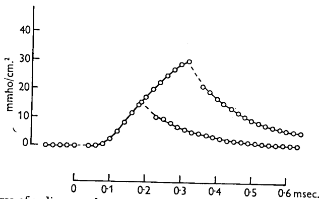
Fig. 5. Time course of sodium conductance estimated from records C and D (Fig. 2) by method described in text. At zero time the membrane potential was reduced by 97.5 mV. and was restored to its resting value at 0.19 msec. (lower curve) or 0.32 msec. (upper curve). The broken part of the curve has been interpolated in the region occupied by the capacitive surge. Axon 41; temperature 3.5° C.; compensated feed-back; V_{Na} = -117 mV.
