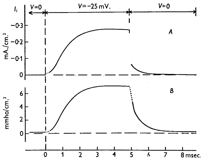
Fig. 13. A , ionic current associated with depolarization of 25 \text{ mV.} lasting 4.9 \text{ msec.} Axon 18 in choline sea water at a temperature of 21^\circ \text{ C.} The curve is a direct replot of the original current record except in the regions 0-0.3 \text{ msec.} and 4.9-5.2 \text{ msec.} , where corrections for capacity current were made by the usual method. Outward current shown upward. B , potassium conductance estimated from A by the equation g_K = I_K / (V - V_K), where V_K is 12 \text{ mV.} and I_K is taken as the ionic current ( I_i ) minus a leakage current of 0.5 \text{ m.mho/cm.}^2 \times (V + 4 \text{ mV.})
