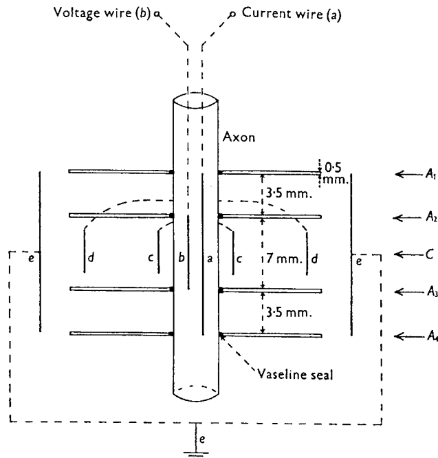
Fig. 1. Diagram illustrating arrangement of internal and external electrodes. A_1, A_2, A_3 and A_4 are Perspex partitions. a, b, c, d and e are electrodes. Insulated wires are shown by dotted lines. For sections through A and C , see Figs. 2 and 3.
