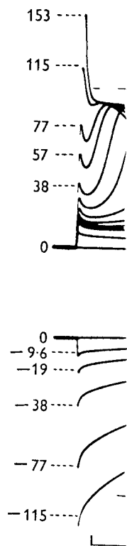
Fig. 8. Time course of membrane current density shown upwards. Axon diameter 400 \mu . Current density 1 \mu coulomb/cm. 2 . Shown downwards.
