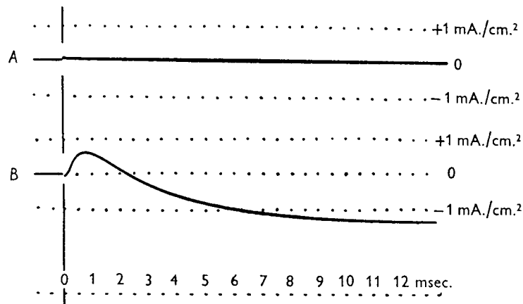
Fig. 11. Records of membrane current under a voltage clamp. At zero time the membrane potential was increased by 65 mV. (record A) or decreased by 65 mV. (record B); this level was then maintained constant throughout the record. Inward current is shown as an upward deflexion. Axon 41; diameter 585 \mu . Temperature 3.8° C. Compensated feed-back.
