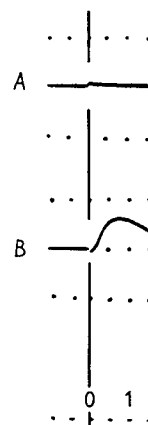
Fig. 11. Records of membrane potential was increased and then maintained upward deflexion. Ax
