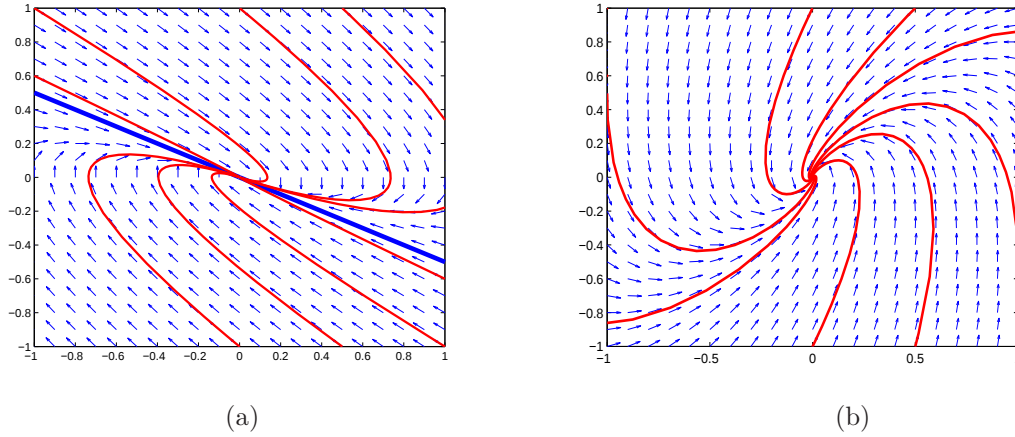
Figure 2.3 Phase portraits. (a) Example 4, (b) Example 5.
