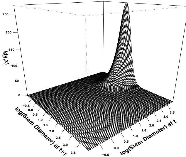
FIGURE 1: The kernel for the Platte thistle integral projection model
