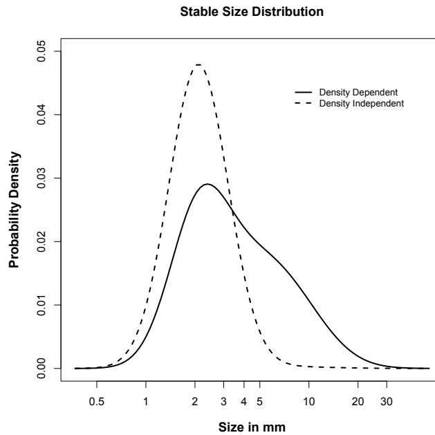
FIGURE 3: Stable state population densities of Platte thistle
