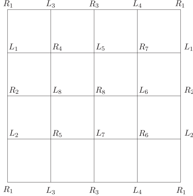
FIGURE 3. The graph \Gamma
