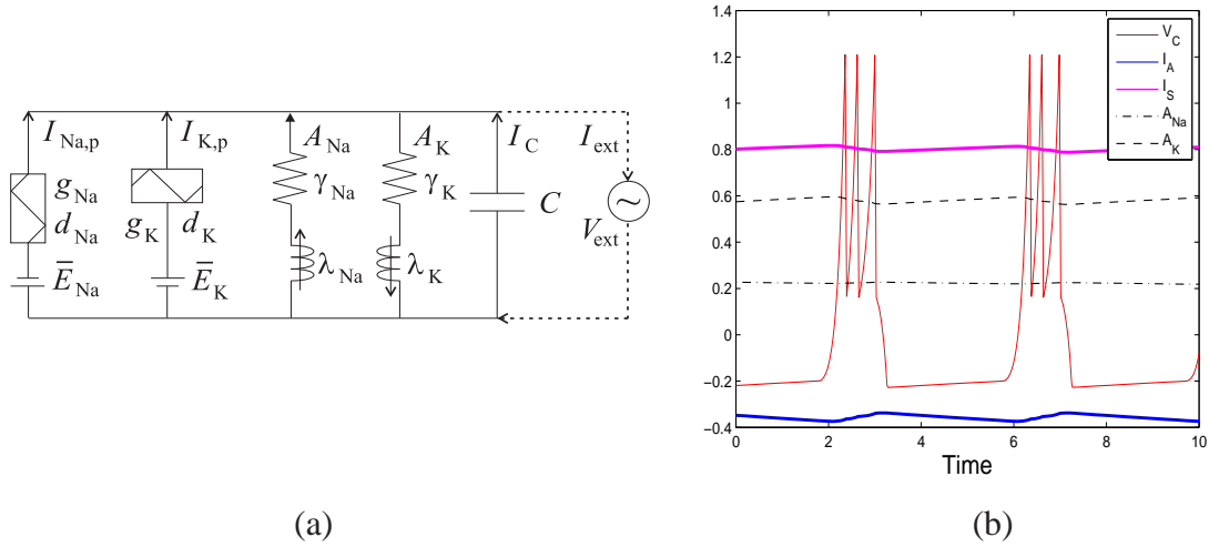
Figure 12: (a) Circuit diagram for the pK_{-d}^+sNa_{+d}^+ type models whose equations are given by Eq.(36). (b) The same parameter values as Fig.10 except for \gamma_{Na} = 0.1 , \gamma_K = 0.05 , \lambda_{Na} = 0.05 , \lambda_K = 0.1 for Eq.(36).
