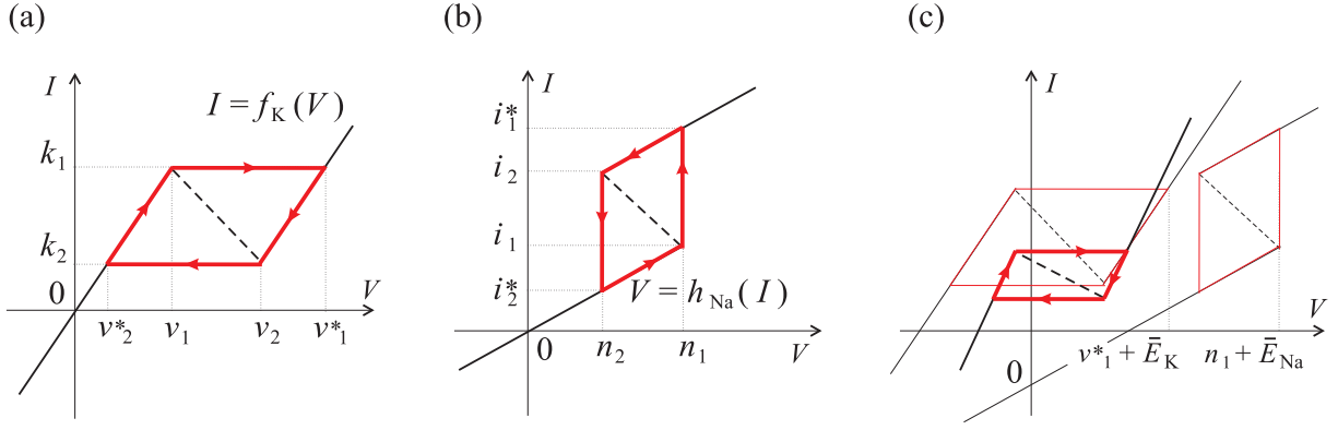
Figure 7: (a) K + 's hysteresis loop of the pK + sNa + model. (b) Na + 's hysteresis loop of the pK + sNa + model. (c) The translated IV-curves by their corresponding passive resting potentials, showing a configuration satisfying condition (27) and condition (28). The new N-hysteresis loop is the result of the vertical sum of K + 's IV-curve and the primary resistive branch of Na + 's IV-curve.
