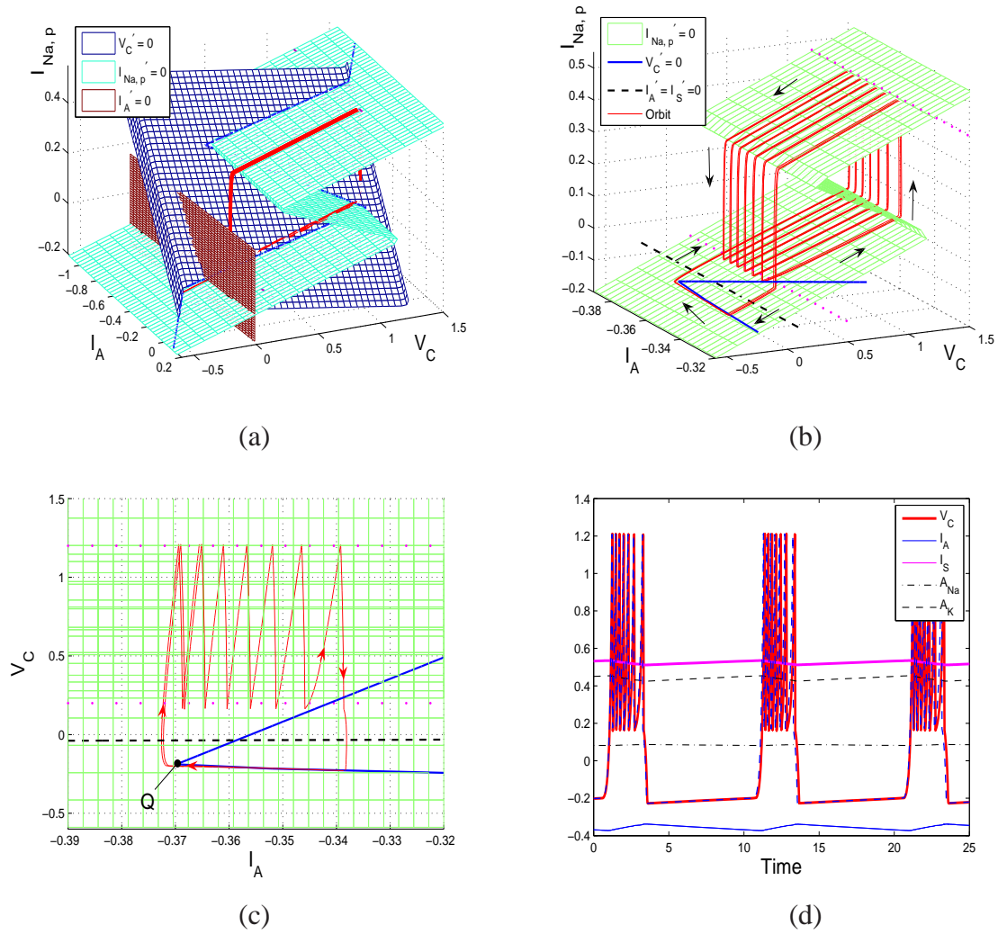
Figure 10: Na + -K + spike-bursts. The same parameter values as Fig.8 except for i_1 = 0.1 , i_2 = 0.3 for which the conditions (32, 33, 34, 35) are satisfied for Eq.(14). For consistence check, the dash spike-burst of (d) tracing the solid spike-burst in variable V_C is generated from circuit Fig.3(c)'s equations from Table 2 with exactly the same parameter values and initial conditions.
